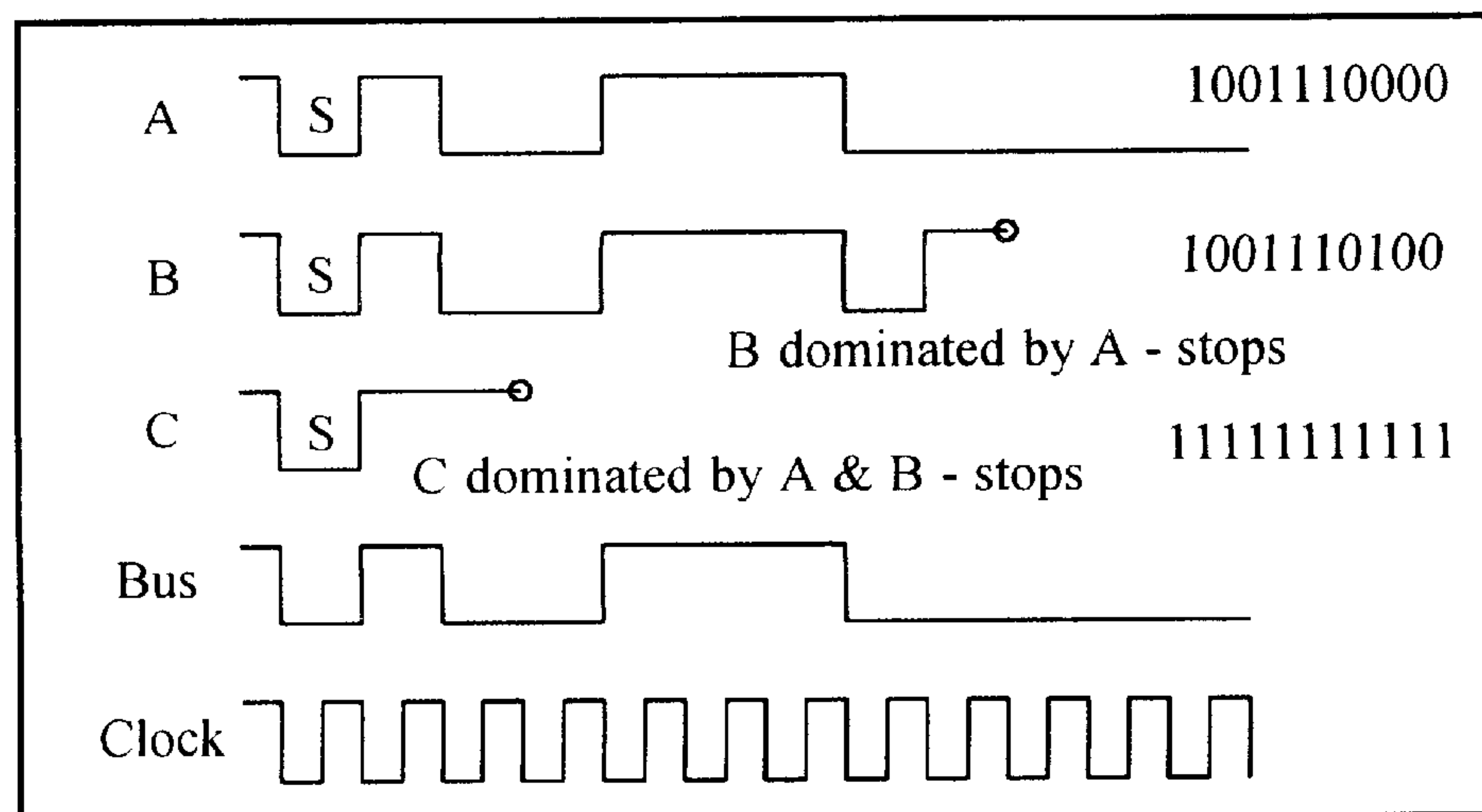
Fig. 2. Example of collision between three messages
