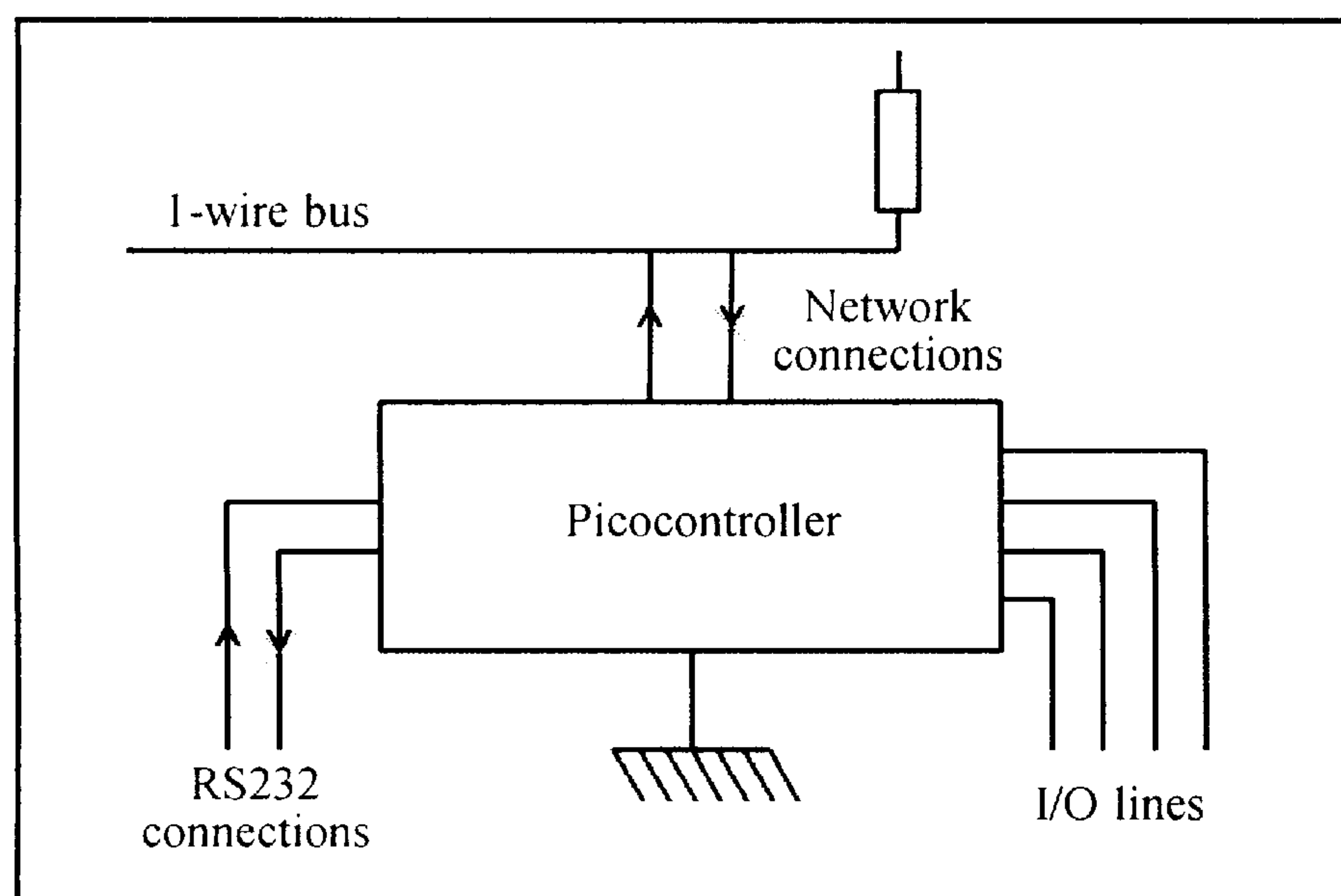
Fig. 5. Three types of connection to the picocontroller
