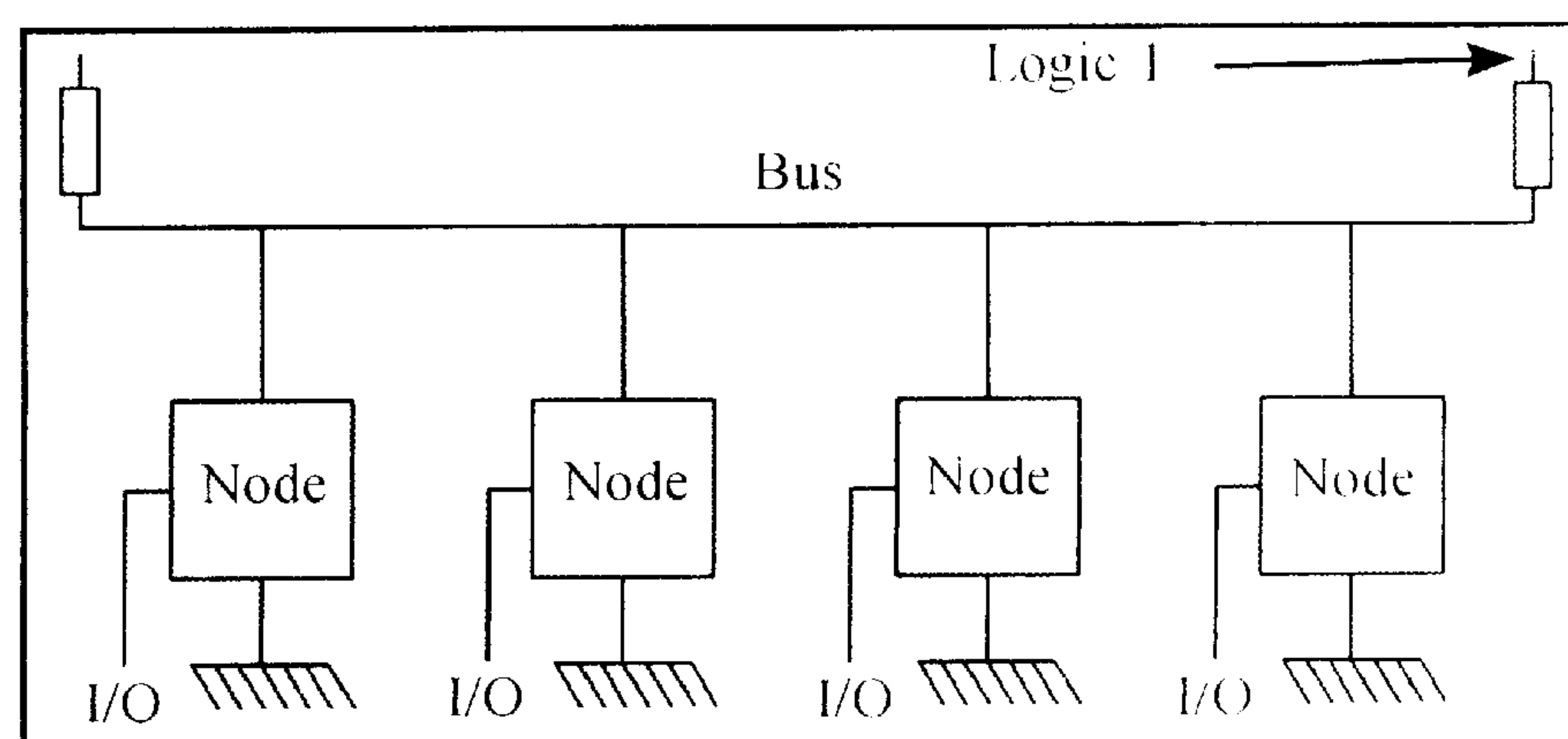
Fig. 1. Basic configuration of One-Wire Network
